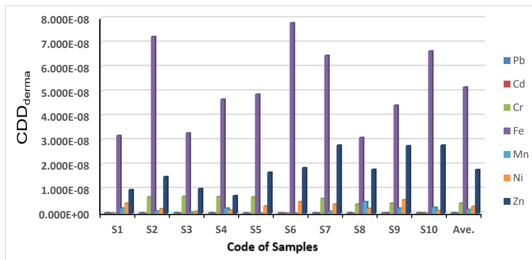
Figure 8. Levels of daily dermal exposure dose (CDD derma ) in different hair dye products.
