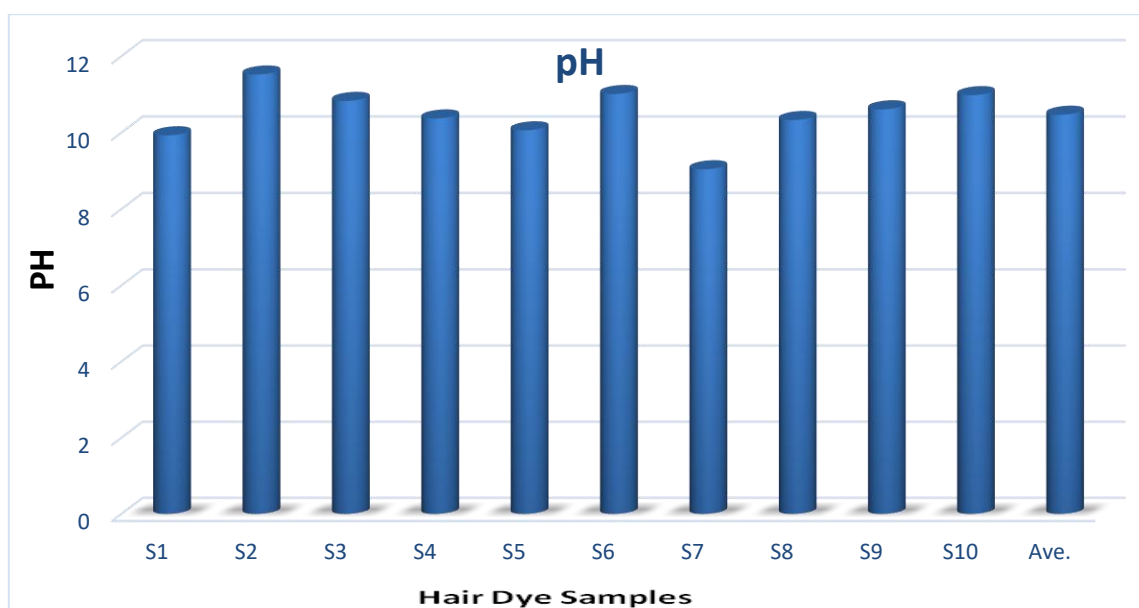
Figure 12. Comparative pH in hair dyes products.
