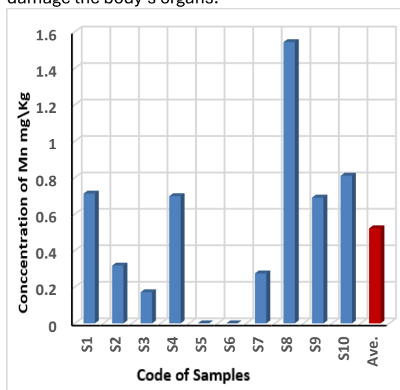
Figure 5. The manganese concentration (mg\Kg) in hair dye samples
