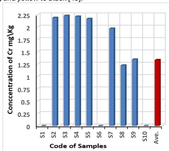
Figure 3. The chromium concentration (mg\Kg) in hair dye samples.
