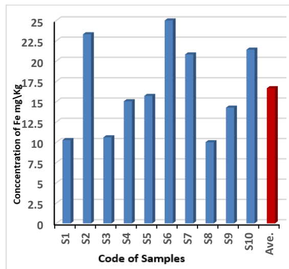
Figure 4. The Iron concentration (mg\Kg) in hair dye samples.
