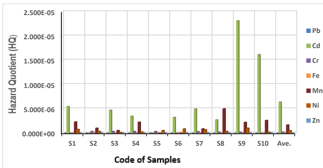
Figure 9. Hazard Quotient (HQ) values for hair dye products.
