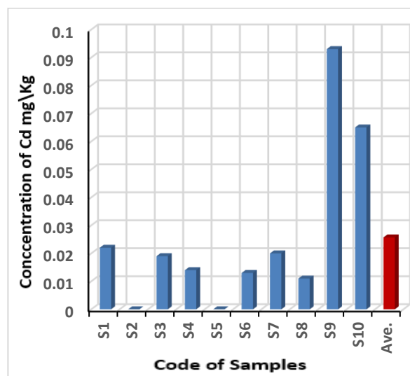
Figure 2. The cadmium concentration (mg/Kg) in hair dye samples
