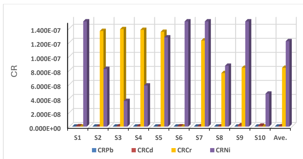
Figure 11. Carcinogenic risk (CR) values for hair dye products.
