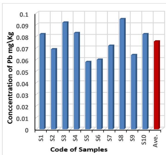
Figure 1. The lead concentration (mg/Kg) in hair dye samples
