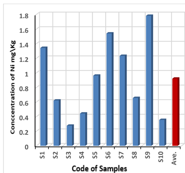
Figure 6. The Nickel concentration (mg\Kg) in hair dye samples.
