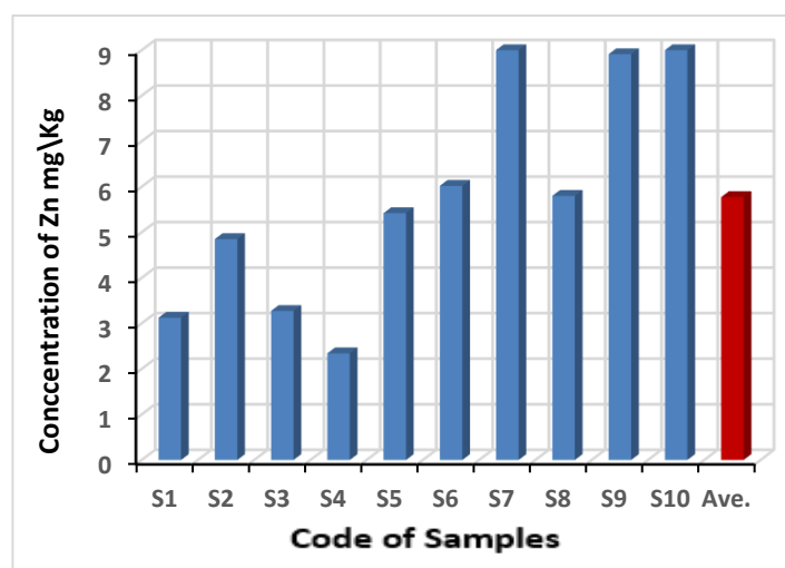
Figure 7. The concentration (mg/Kg) in hair dye samples.
