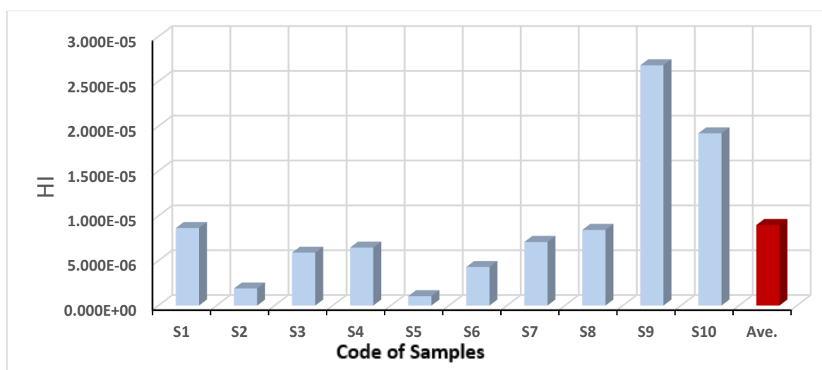
Figure 10. Hazard Index (HI) values for hair dye products.
